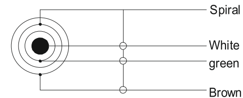
Wiring method
