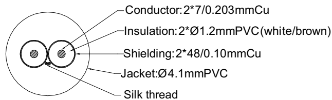
Cable section
