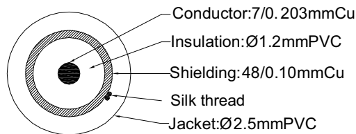
Cable section
