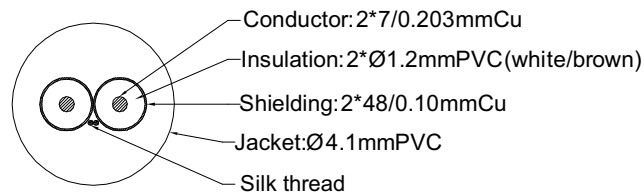
Cable section
