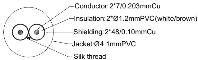
Cable section
