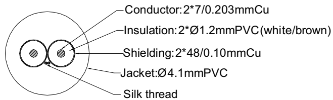
Cable section
