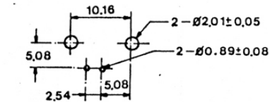
PCB HOLE CONFIGURATION
