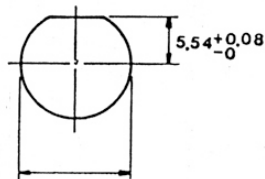
RECOMMENDED PANEL CUTOUTS
