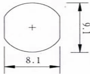
Mounting Holes
