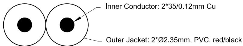
Cable Structure (0.4mm 2 )
