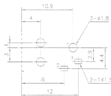
PIN HOLE LAYOUT (BOTTOM VIEW)
