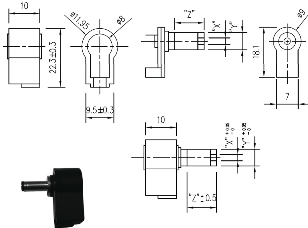
DC PLUG (RIGHT ANGLE TYPE)
