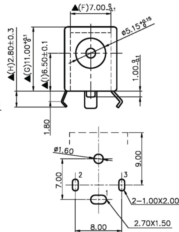
Pin Hole Layout (Jack Bottom View)
