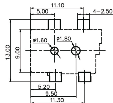
Pin Hole Layout (Jack Bottom View)
