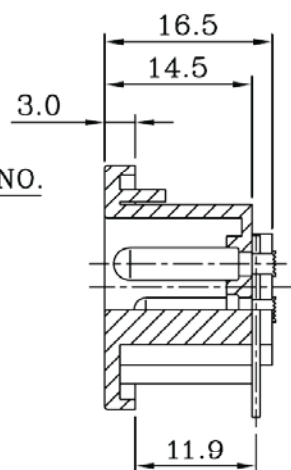
B-B SECTION
