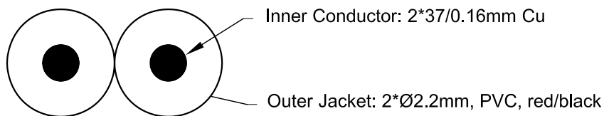
Cable Structure
