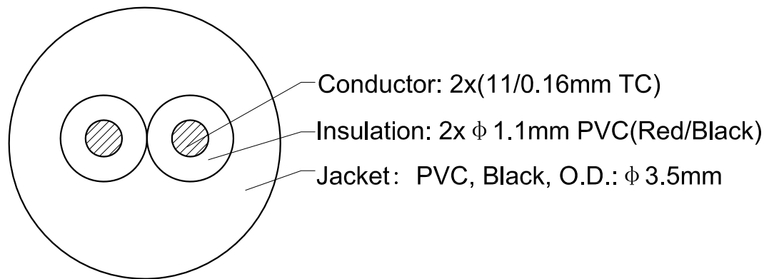
Cable Structure (24AWG*2C)
