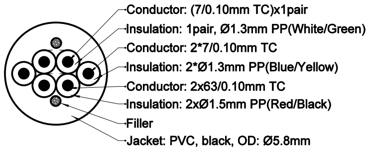
Cable Structure
