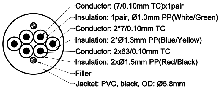
Cable Structure
