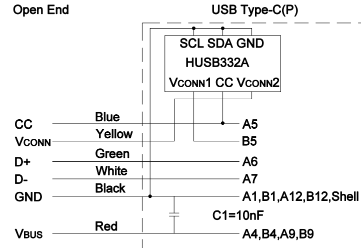
Wiring Diagram
