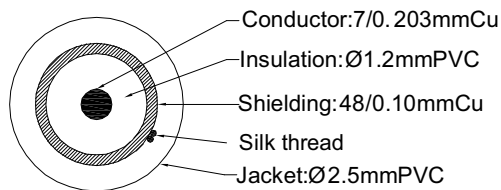
Cable section
