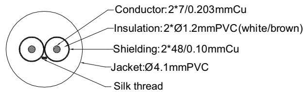
Cable section
