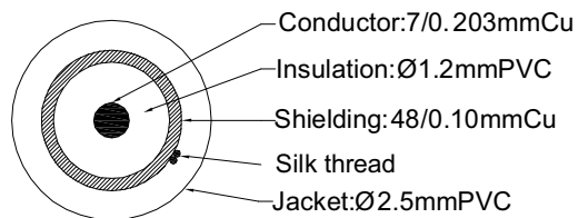
Cable section
