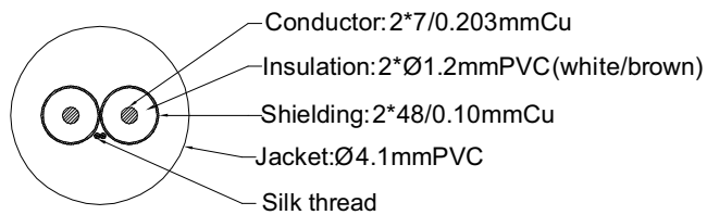
Cable section
