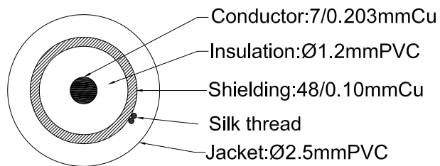
Cable section
