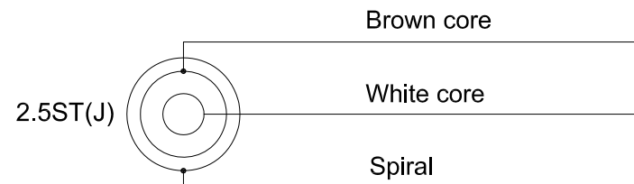
Wire layout
