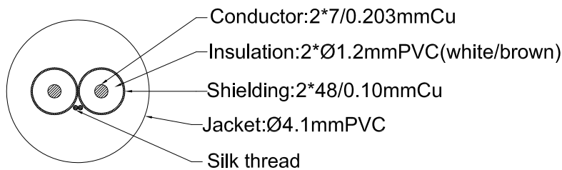
Cable section
