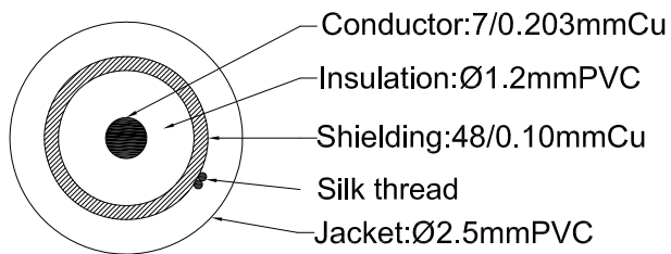
Cable section
